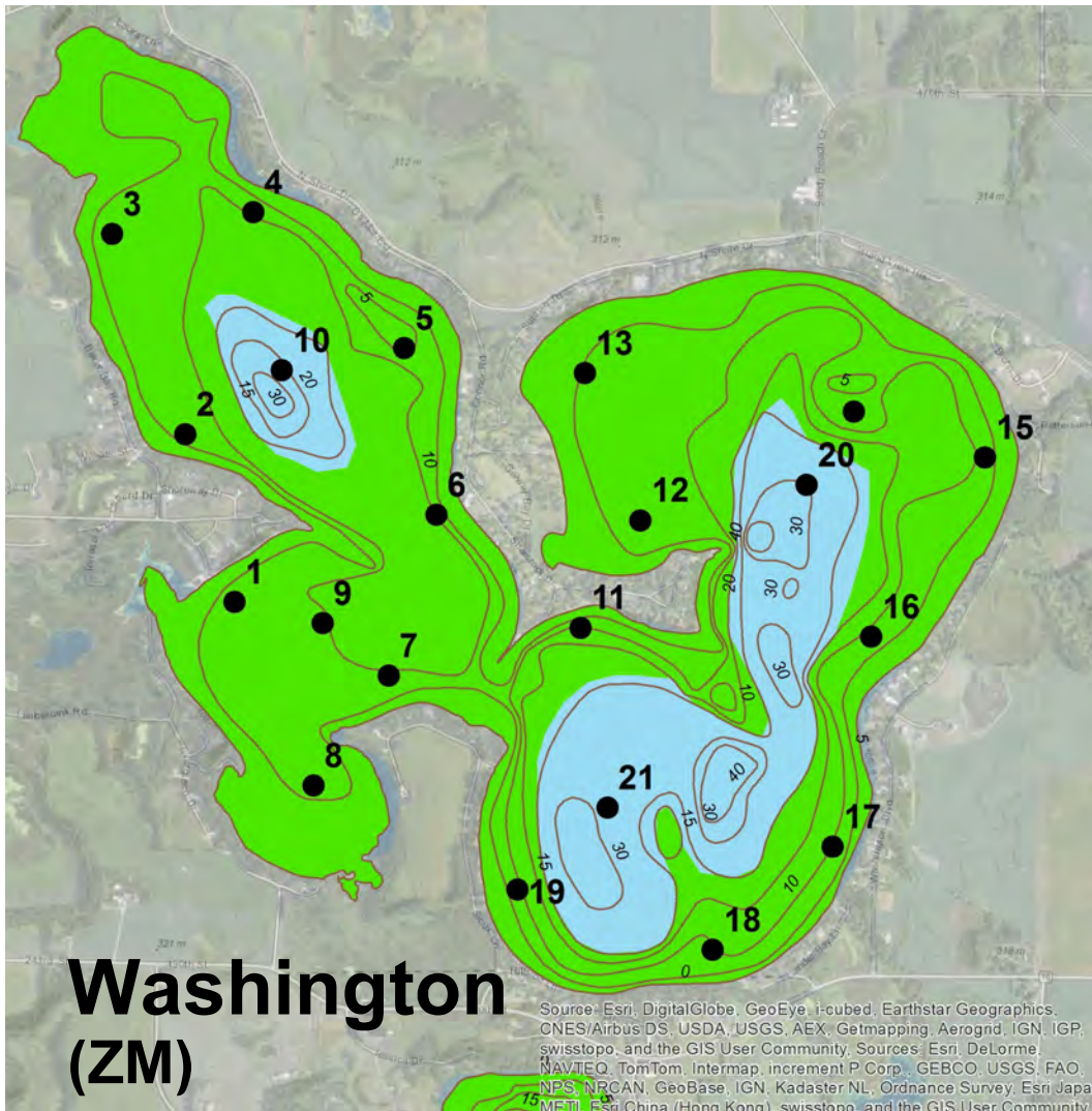
Figure S4. Zebra mussel potential growth based on water column and substrate characteristics. Key for Potential Growth: Green = light growth.
