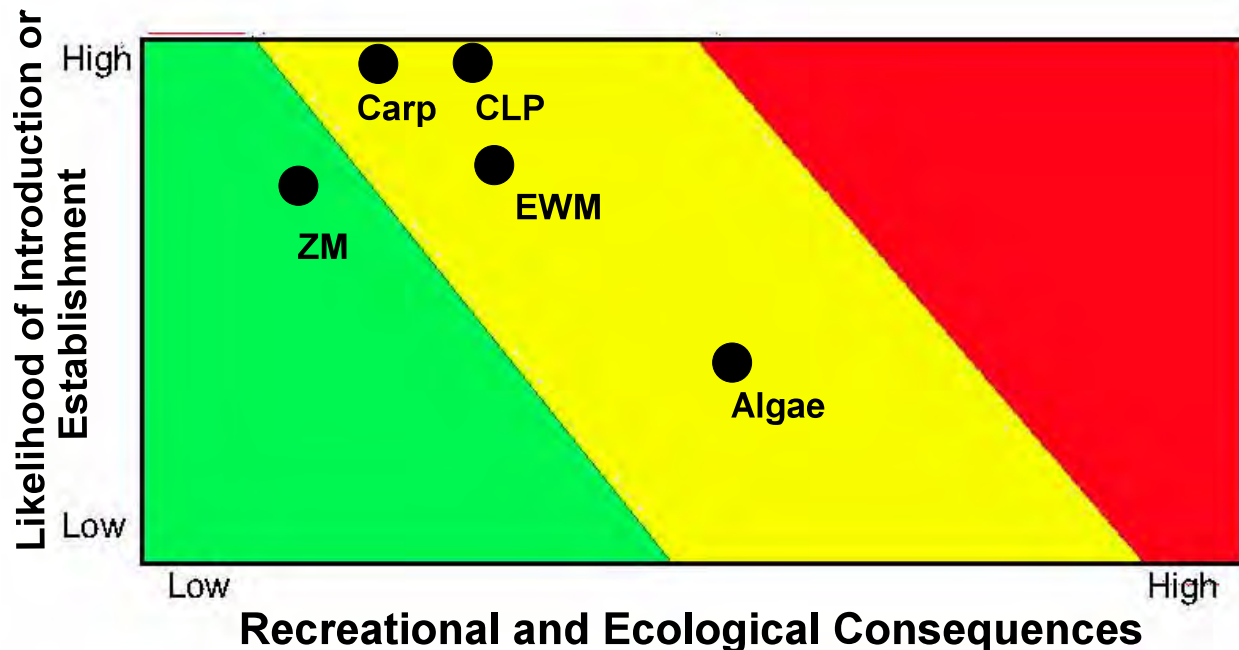
Figure S6. Based on available information, an environmental risk assessment (ERA) chart was prepared for five aquatic invasive species of interest for Lake Washington.
